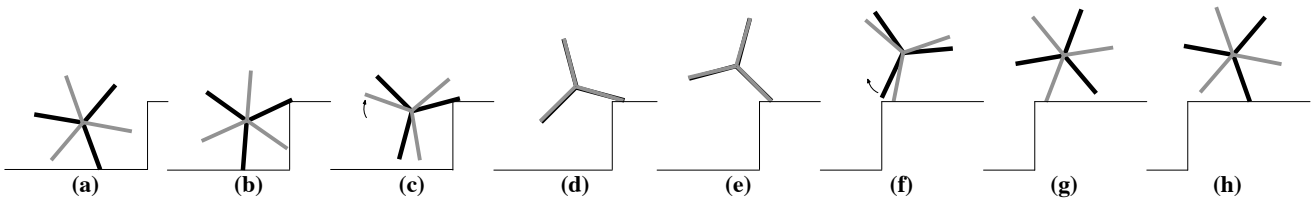
Figure 2. Illustration of the Whegs concept: a) the two front whegs of the robot approach an obstacle; b) the far (black) wheg makes contact first, and c) while the far wheg is slowed, passive torsional compliance in the drive train allows the near (gray) wheg to rotate into phase with the far wheg; d) once in phase, the two whegs can e) propel the front of the robot over the obstacle; f) atop the obstacle the two whegs separate and g) spring back to their h) prior configuration.
